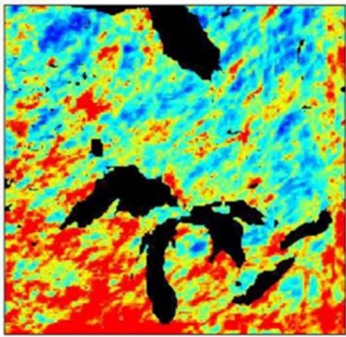
PROJECTED FUTURE CHANGES IN EXTREME RAINFALL IN 2045-2060. D'ORGEVILLE AND PELTIER 1 , JGR – ATOMS. 2014 UNIVERSITY OF TORONTO
