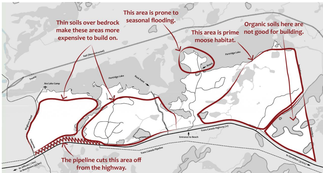
SAMPLE FLOOD MAPPING USED IN LAND-USE PLANNING HTTPS://WWW.CIP-ICU.CA/PDF/2013-26-GIIWEDAA-PARTRIDGE-LAKE-LAND-USE-PLAN.PDF
